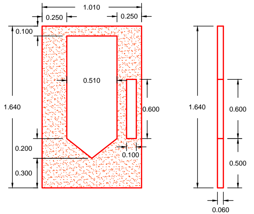
D FRONT ELEVATION
