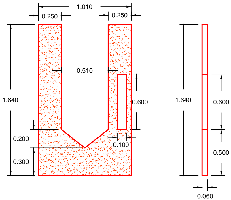
B FRONT ELEVATION
