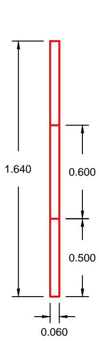
SIDE ELEVATION
